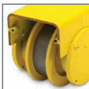
Removable Rail Sweeps for access to wheels
